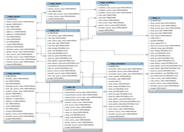
Figure 1. ETL Staging Tables
